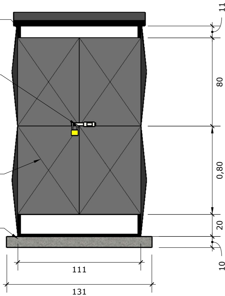
VISTA FRONTAL
